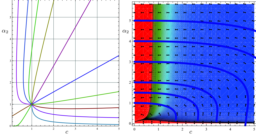
Fig. 3. Geodesics passing through (c, \alpha_2) = (1, 1) (left) and a contour plot of the entropy with some integral gradient curves (right), in the McKay submanifold M_1 which has \alpha_1 = 1 .
