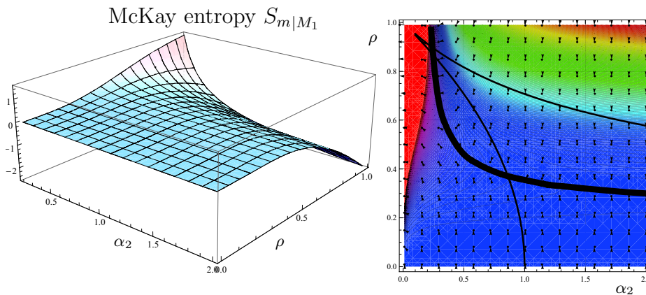
Fig. 4. Surface representation of the Shannon entropy function S_m for the submanifold M_1 of the McKay family with respect to parameter \alpha_2 and correlation coefficient \rho (left), and contour plot (right). Superimposed also are gradient flow arrows and the thick curve is the locus of maximum entropy. The two thinner curves show the loci of \alpha_1 = 1 (upper curve) and \alpha_1 + \alpha_2 = 1 (lower curve), which correspond, respectively, to Poisson random processes for the X and Y variables.
