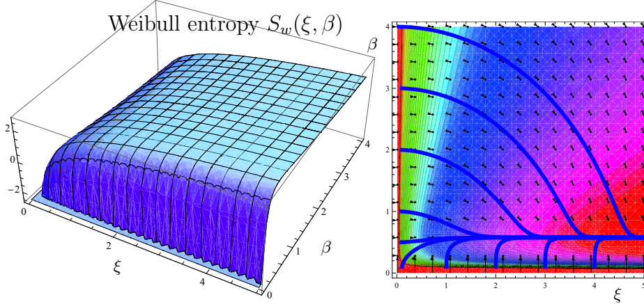
Fig. 5. Surface representation of the Shannon entropy function S_w for the Weibull family (left), and contour plot (right) with gradient flow and integral curves.
