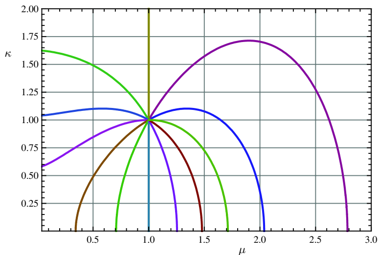
Fig. 1. Some examples of maximally extended geodesics passing through (\mu, \kappa) = (1, 1) in the gamma 2-manifold.
