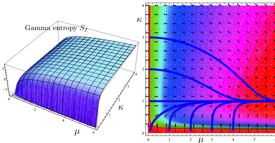
Fig. 2. Shannon entropy function S_f for the gamma family as a surface with respect to mean \mu and \kappa (left) and as a contour plot with entropy gradient flow and integral curves (right). The asymptote is \kappa = 1 , the exponential case of maximum disorder.
